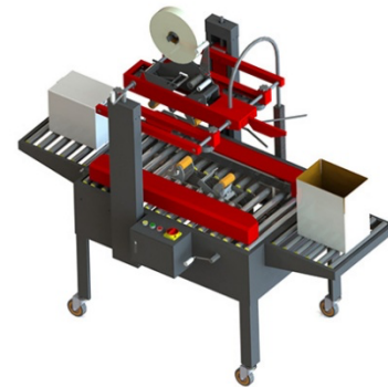
In Line Box closer + Double Tape Sealer CS35
